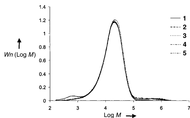
Figure 3. Molecular-weight distribution from GPC analysis of the polymers obtained with complexes 1–5 as precatalysts.
