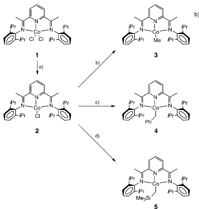
Scheme 1. Synthesis of [\text{N}_3^{\text{iPr}}\text{Co}^{\text{I}}] complexes. Reagents and conditions: a) 1.2 equiv MeLi, toluene, 5 h or 2 equiv MAO, toluene, instant; b) 1.1 equiv MeLi, diethyl ether, 3 days or 2 equiv MAO, toluene, instant; c) 2.0 equiv \text{Bn}_2\text{Mg} , toluene, 2 h; d) 1.2 equiv \text{LiCH}_2\text{SiMe}_3 , toluene, 10 min.
